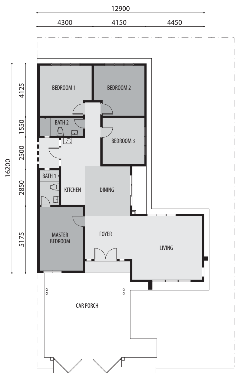
Floor Plan
